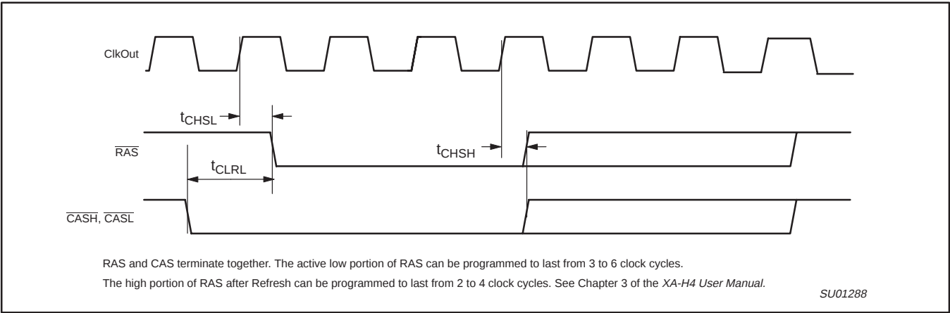
Figure 21. REFRESH
