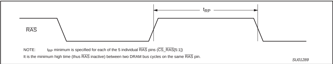
Figure 22. RAS Precharge Time
