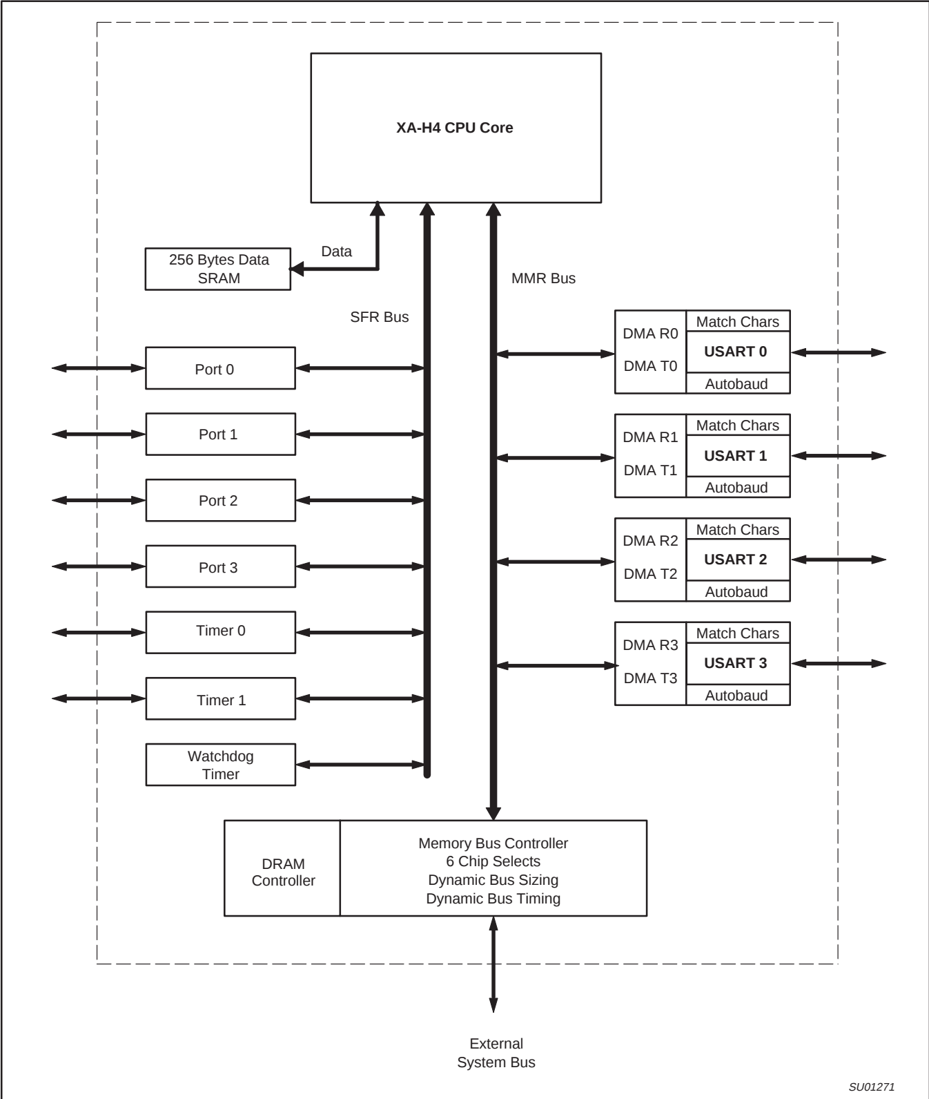
XA-H4 BLOCK DIAGRAM
